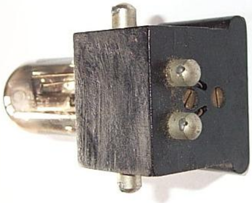
Above is the I/S4 interservice base. This valve carries the serial number A951. It was made by MOV.
